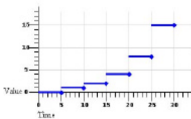
Fig.1: discrete function
